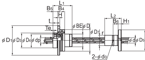
Ball screw unit (Models NS 0812A and 1015A) Ball spline (Models NS 0812A and 1015A) Ball spline (Models NS 0812A and 1015A)
