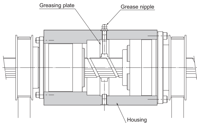
Fig.6 Lubrication Methods
