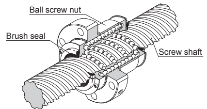
Brush seal
