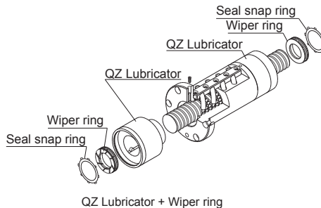
QZ Lubricator + Wiper ring
