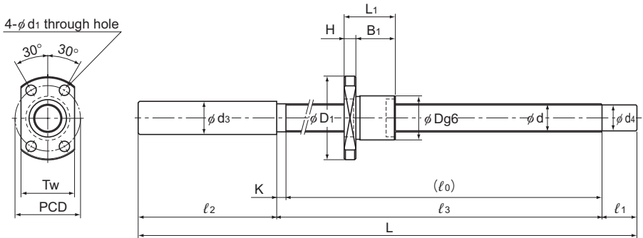
Model MDK
