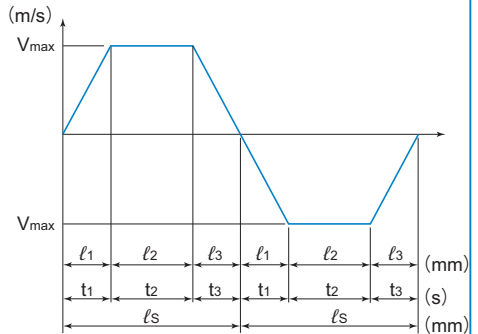
Velocity diagram
